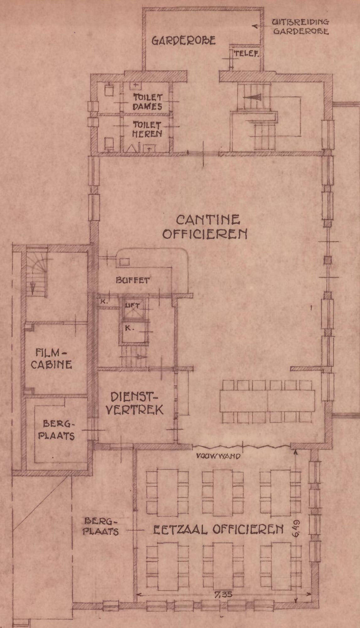
PLAN VERDIEPING
